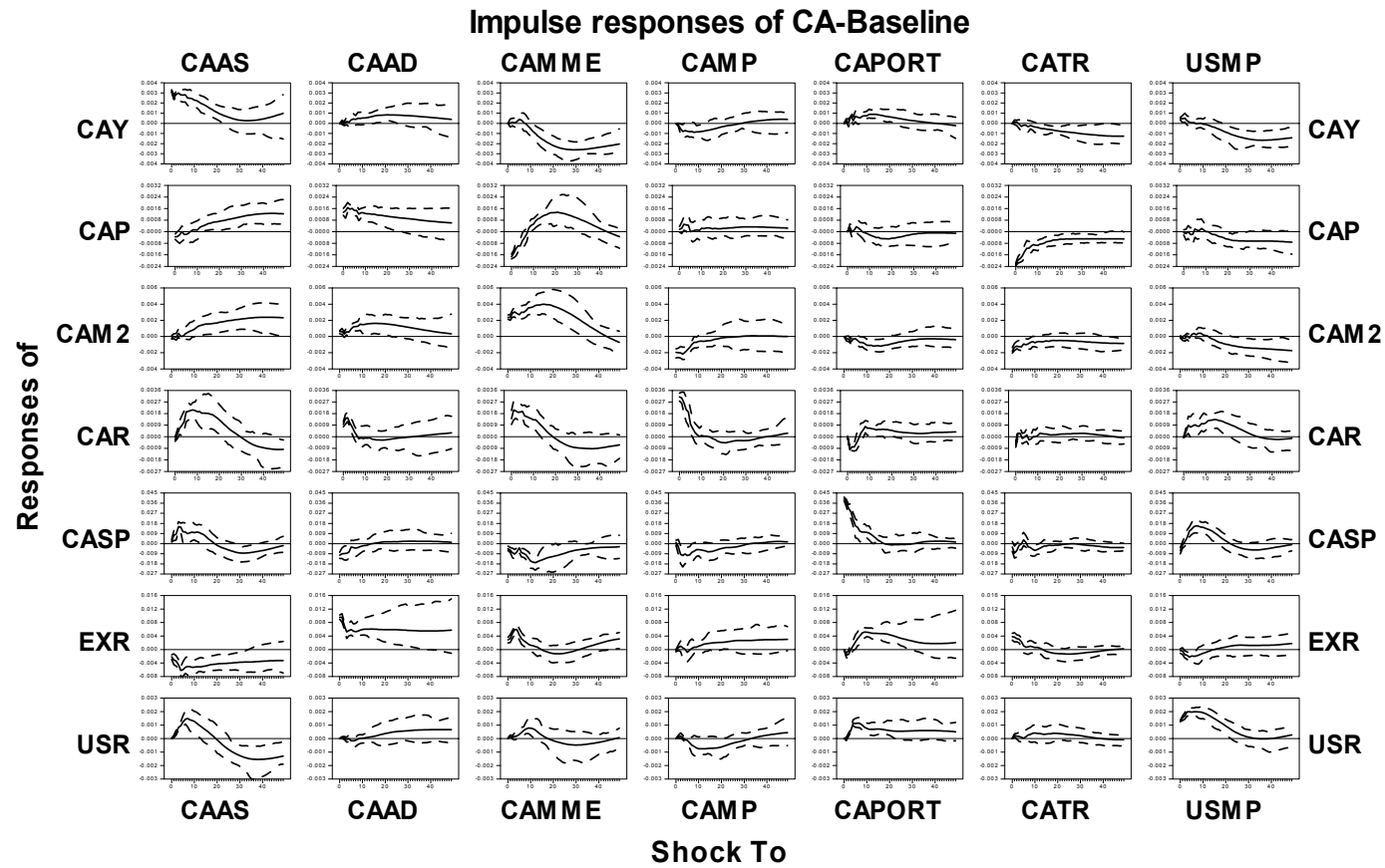
Figure 2. Dynamic responses to structural shocks in the baseline Canadian model with short-run restrictions as in equation (10) (intervals between the dashed lines correspond to two standard errors)
